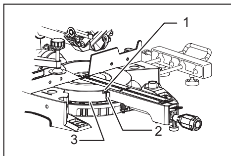
► 1. Screw 2. Pointer 3. Miter scale
