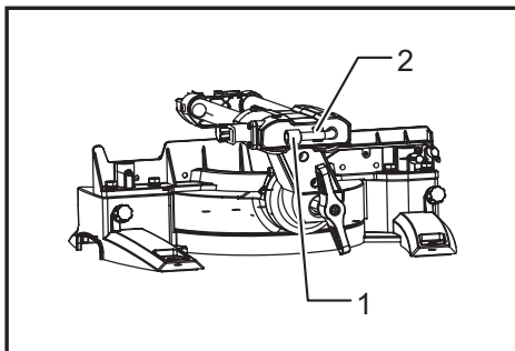
► 1. Socket wrench with hex wrench on its other end 2. Wrench holder
